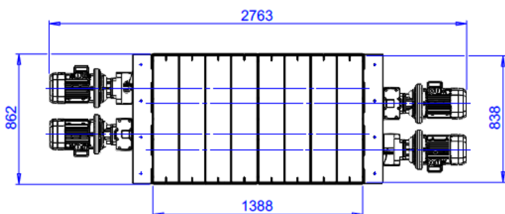
Cutting block DELOS-1400
