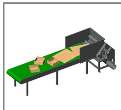
DELOS-1400 horizontal introduction by conveyor
