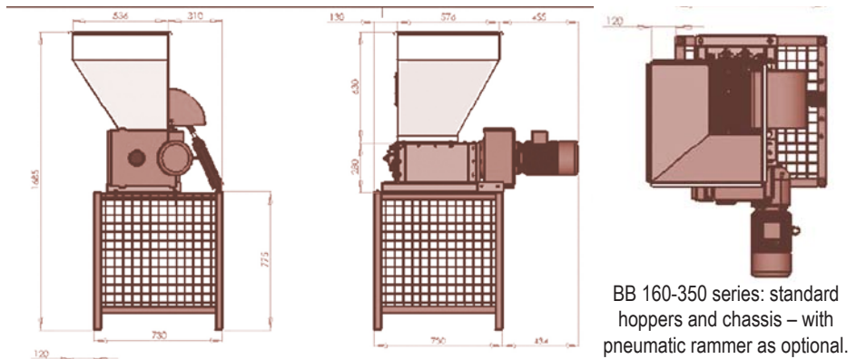
BB230 BLiK crusher: with pneumatic rammer: for plastic bottles. Handles 500-600 per hour.
